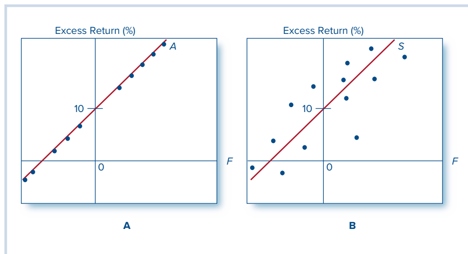
Figure 10.2 Excess returns as a function of the systematic factor: Panel A , Well-diversified portfolio A; Panel B , Single stock (S).
