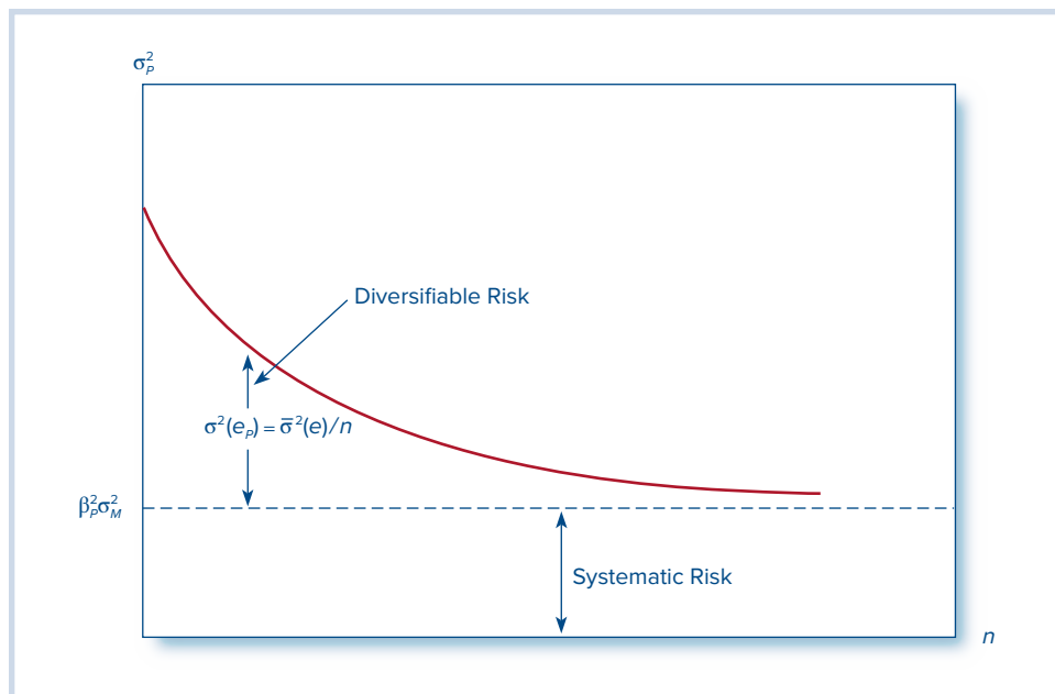
Figure 8.2 The variance of an equally weighted portfolio with risk coefficient \beta_p in the single-index economy as a function of the number of firms included in the portfolio
