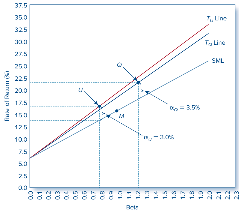
Figure 24.3 Treynor measures of two portfolios and the market index
