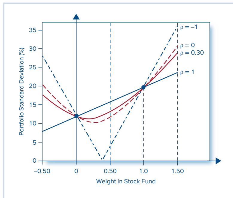
Figure 7.4 Portfolio standard deviation as a function of investment proportions
