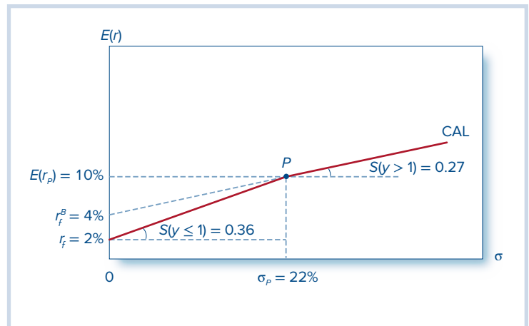
Figure 6.4 The investment opportunity set with different borrowing and lending rates
